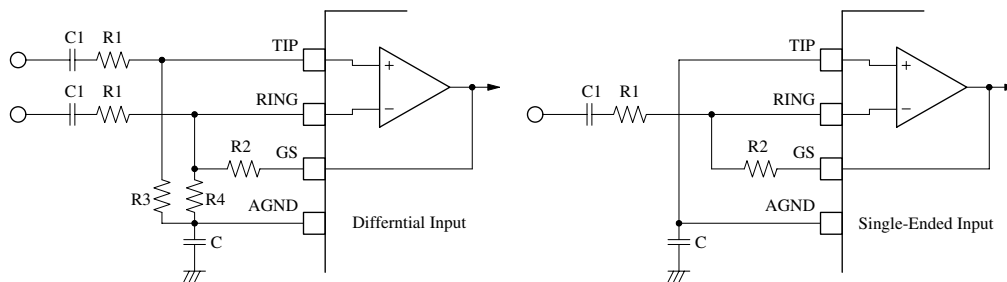
Figure 3. Input circuits
