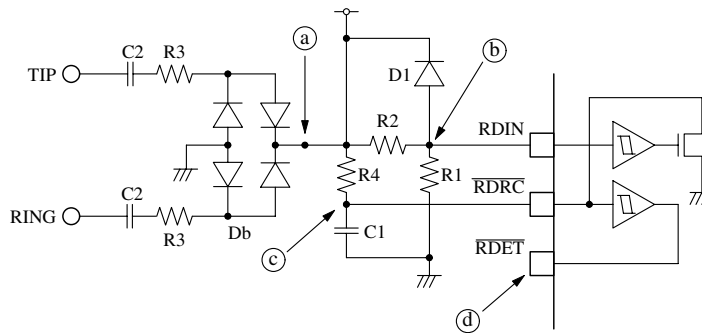
Figure 1. Ring signal detector circuit
