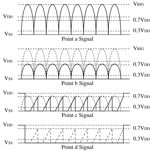
Figure 2. Ring signal detector circuit waveform transitions
