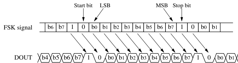
Figure 4. FSK signal to DOUT output
