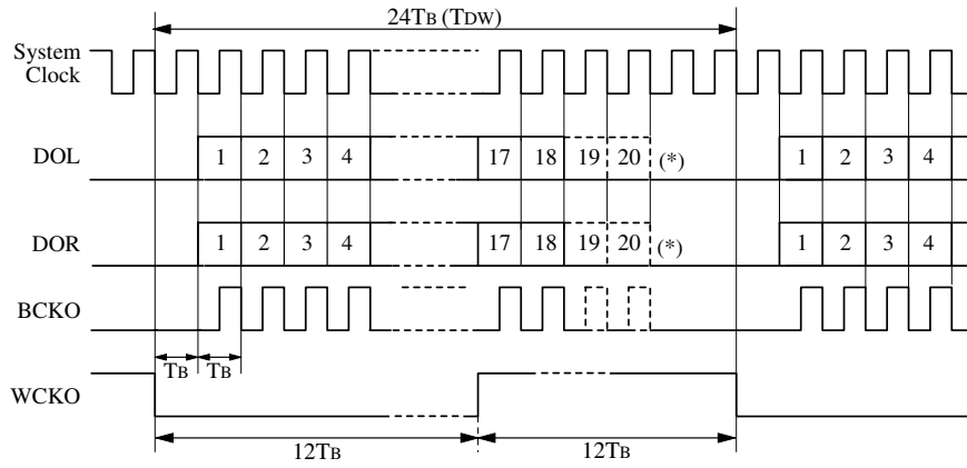
Figure 10. 18/20-bit output ( \overline{\text{CKSL}} = \text{HIGH} )
