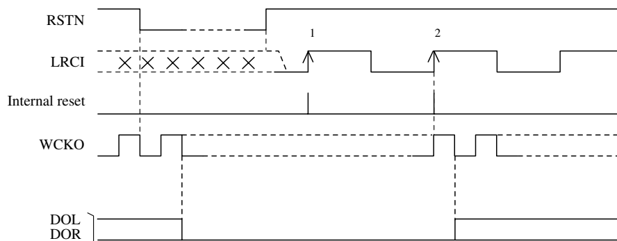
Figure 6. System reset timing and output muting
