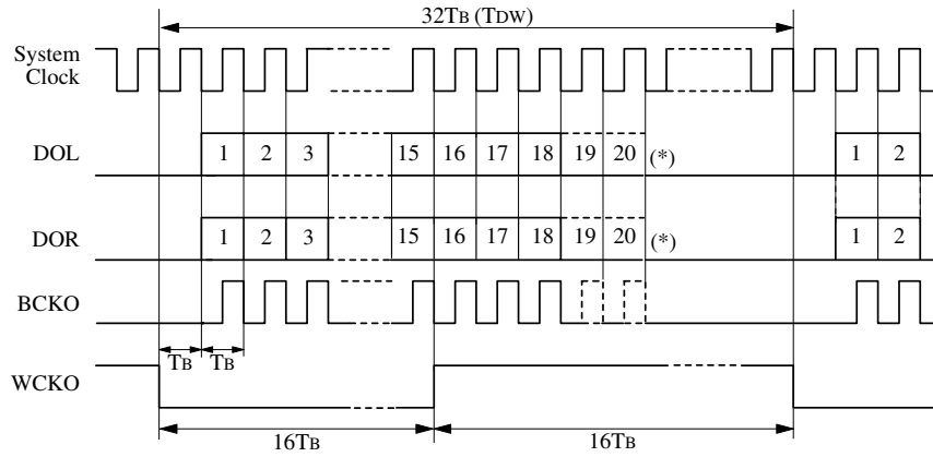
Figure 11. 18/20-bit output ( \overline{\text{CKSL}} = \text{LOW} )
