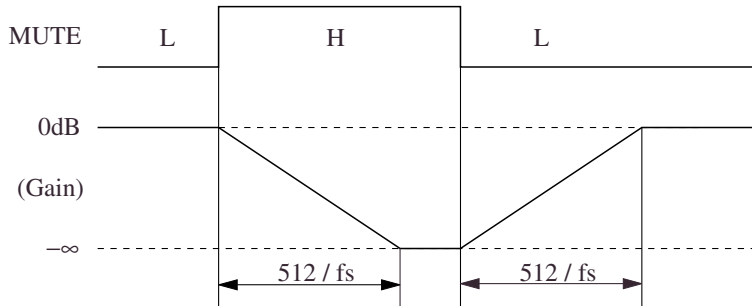
Figure 2. Mute timing
