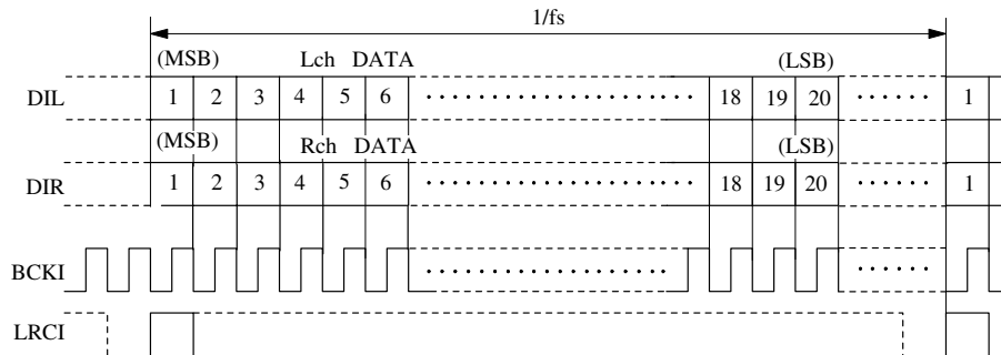
Figure 8. LR alternating, leading data, 20-bit input
