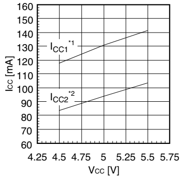
Figure 23. I_{CC1} vs. V_{CC} (6dB, FCDATA = 255) *1. filter mode, FCDATA = 255 *2. filter bypass mode
