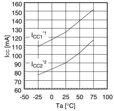
Figure 24. I_{CC1} vs. T_a (6dB, FCDATA = 255) *1. filter mode, FCDATA = 255 *2. filter bypass mode
