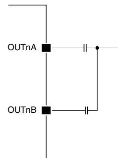
Figure 5. Connection with sag compensation circuit
