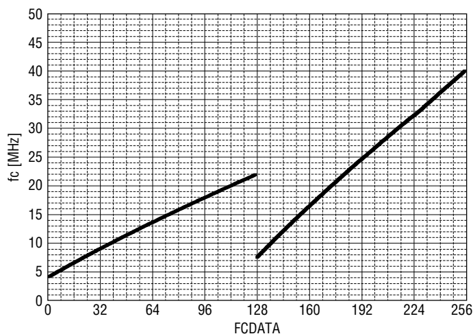
Figure 1. Cutoff frequency vs. FCDATA ( R_{ISET} = 1.8k\Omega )
