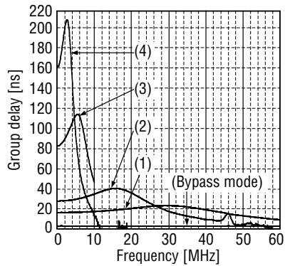
Figure 16. Group delay vs. FCDATA, fc mode
