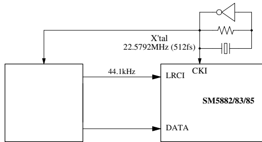
2-wire input type System clock 512fs
