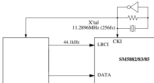
2-wire input type System clock 256fs
