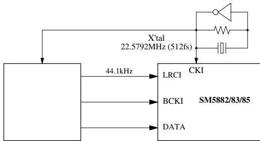
3-wire input type System clock 512fs
