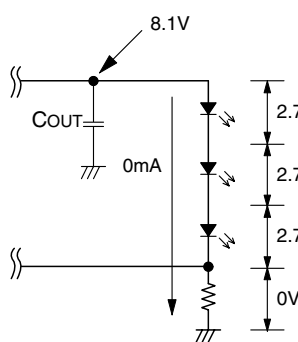
Output voltage with LEDs OFF
