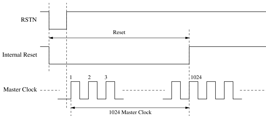
Figure 3. External reset timing
