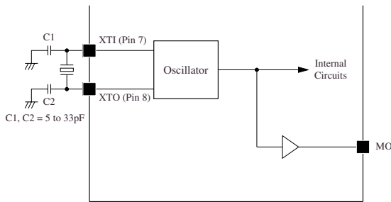
Figure 3. Crystal oscillator connection (excluding SM8707J)
