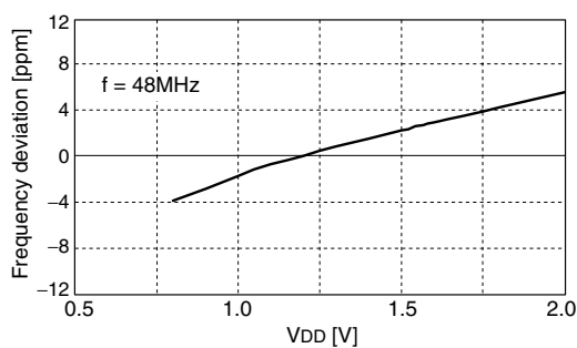
5028×1, C_L = 15\text{pF} , 1.2V standard, T_a = 25^\circ\text{C}
